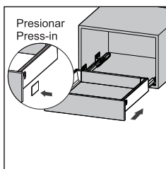
Deslizar dentro del gabinete Slide into the cabinet
