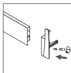
Ensamble frontal Front panel assembly
